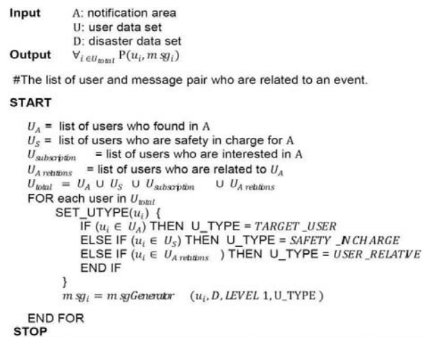
Figure 3. Knowledge based Message Generation Algorithm user involved in an event.
