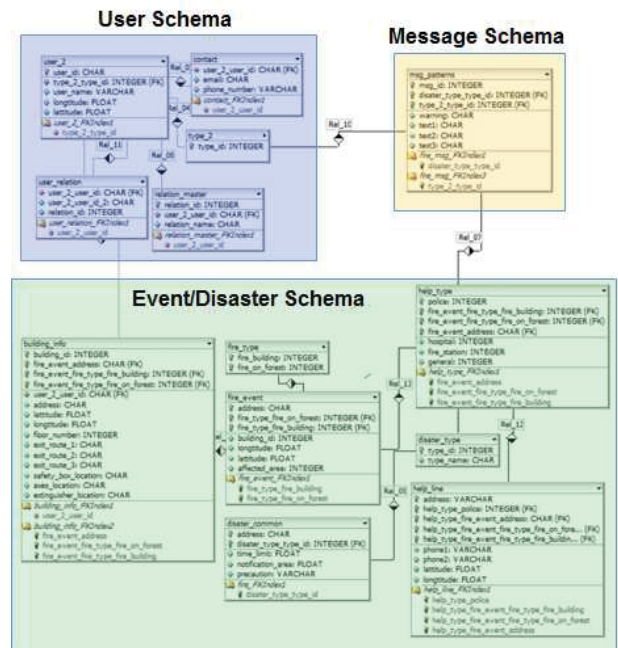
Figure 2. Design of the database
