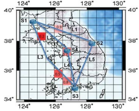
Figure 4. An example of mapping location trustiness and a network topology to GMM
